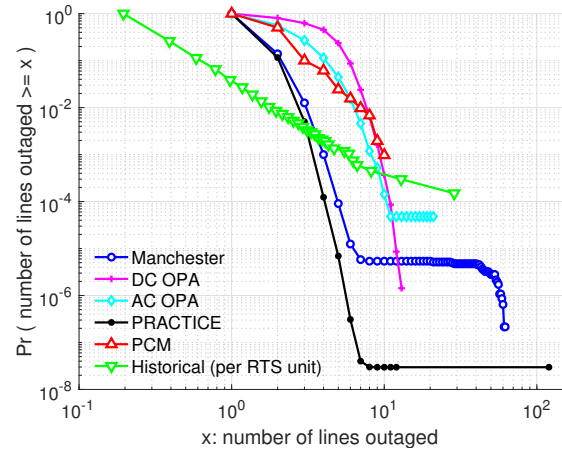
Fig. 4. Distribution of number of lines outaged
